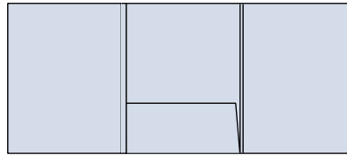
623 Style 9" x 12" x 1/8" three panel design with one glued 4" pocket in the center panel.
