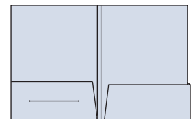
9472 Style 9" x 12" with one 4" high, 3/8" box pocket and one 4" high flat pocket.
