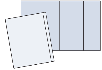
9533 Style 9 3/4" x 11 3/4" with one 4" wide vertical pocket. Back panel is 3/4" wider than front cover to provide a 3/4" tab extension.
